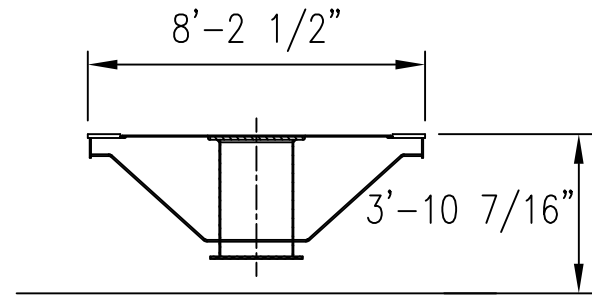
SECTION AT CENTER X-BEARER
